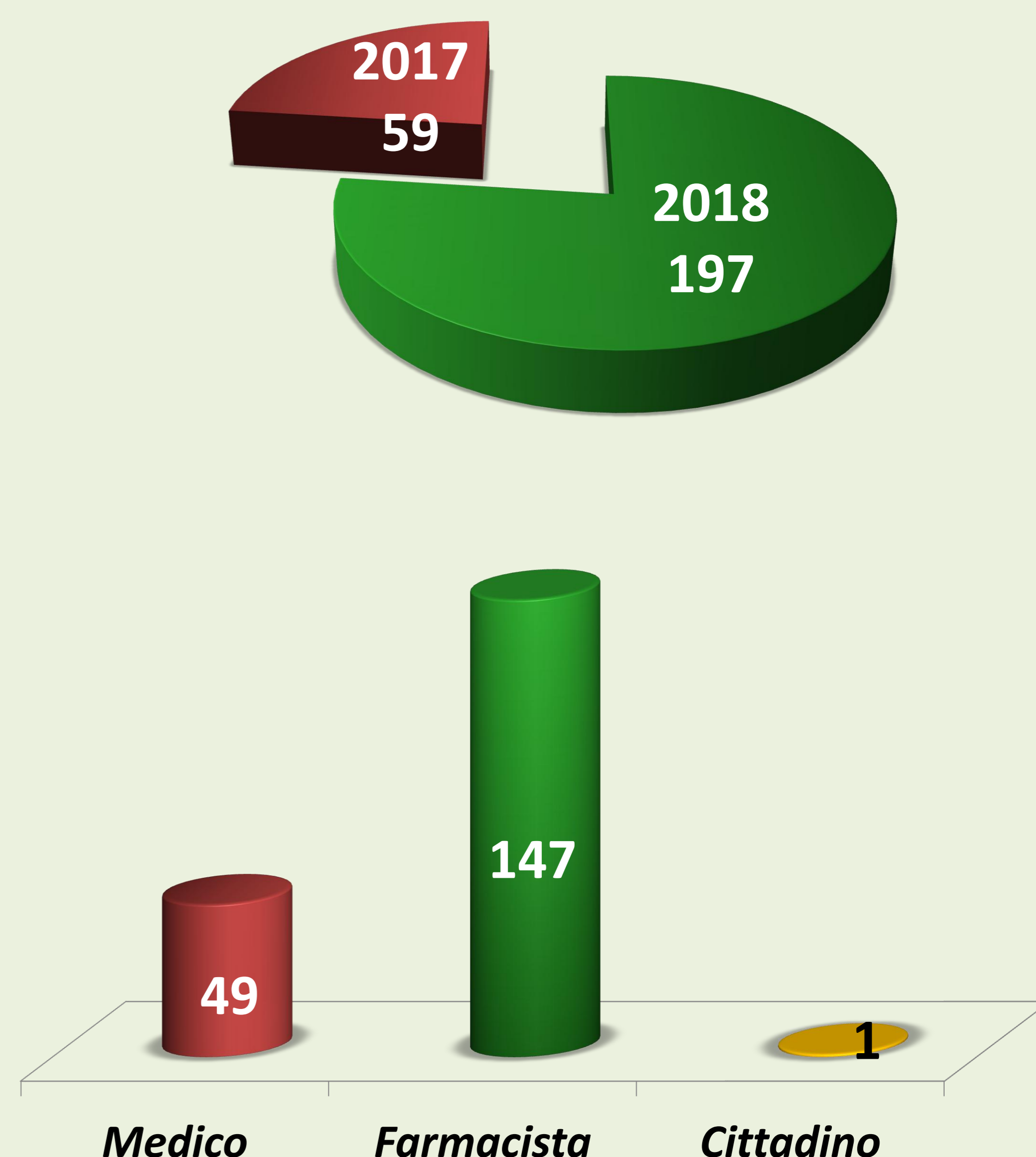
ADR 2018 vs 2017
